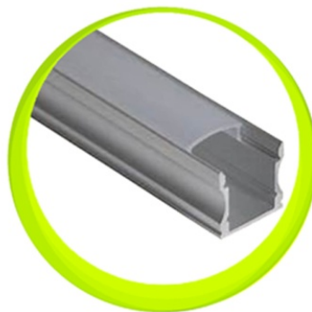
LED Linear light Model No.- 10X13mm Surface colour- white/ NW /warm white Size- 10X12.9mm, Lenth- 2 MTR
